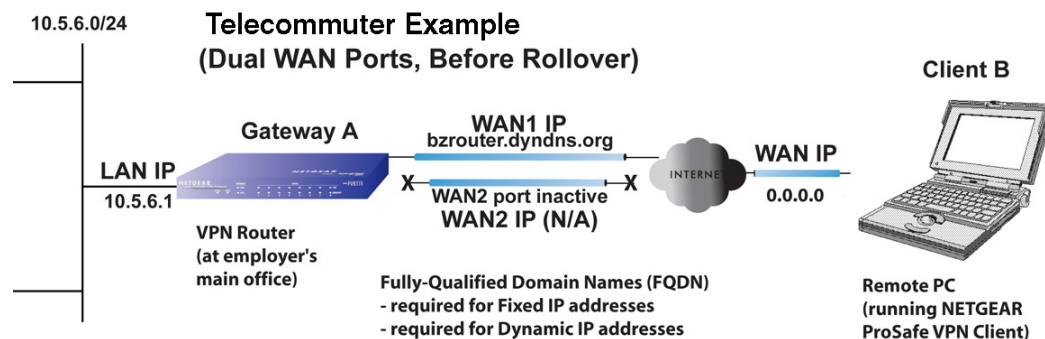
Figure 21. Telecommuter example in a dual WAN port configuration before auto-rollover
