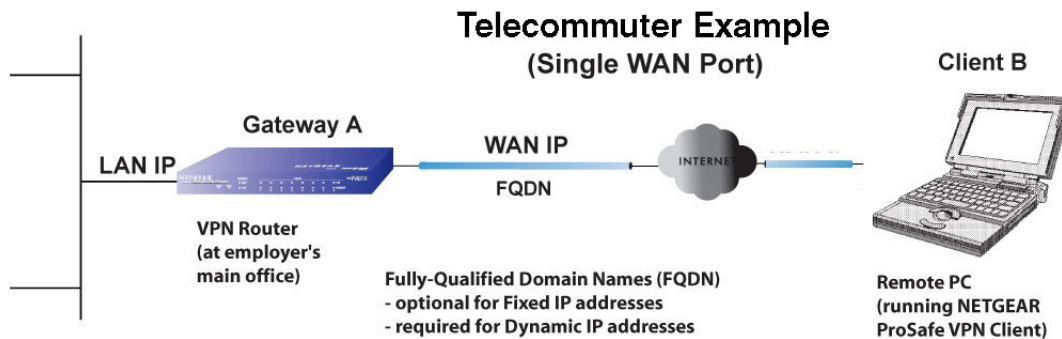
Figure 9. Example of an IPv4 client-to-gateway IPSec VPN connection
