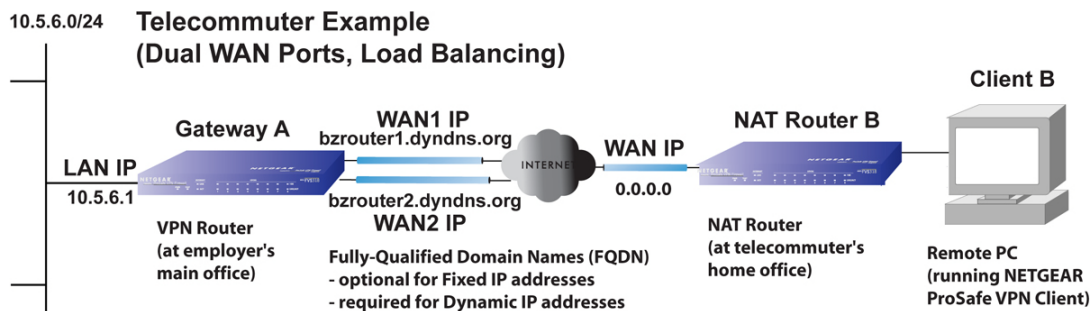
Figure 31. Telecommuter example in a dual WAN port configuration with NAT and load balancing
