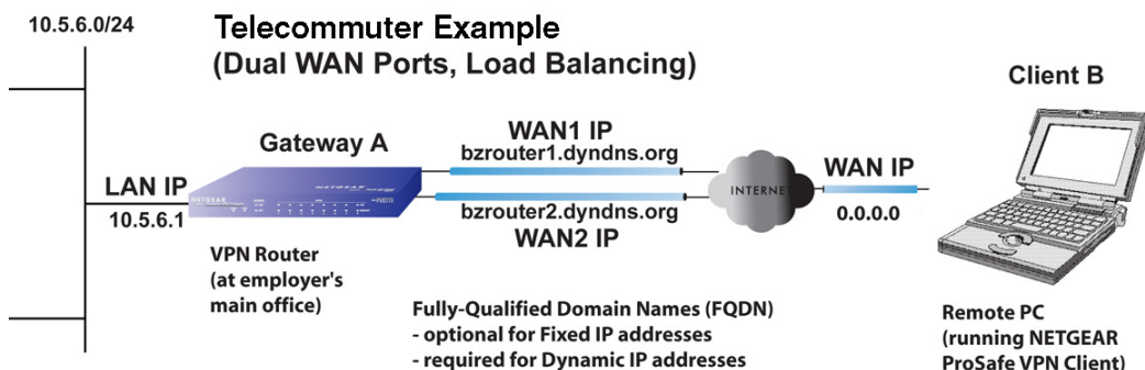
Figure 23. Telecommuter example in a dual WAN port configuration with load balancing
