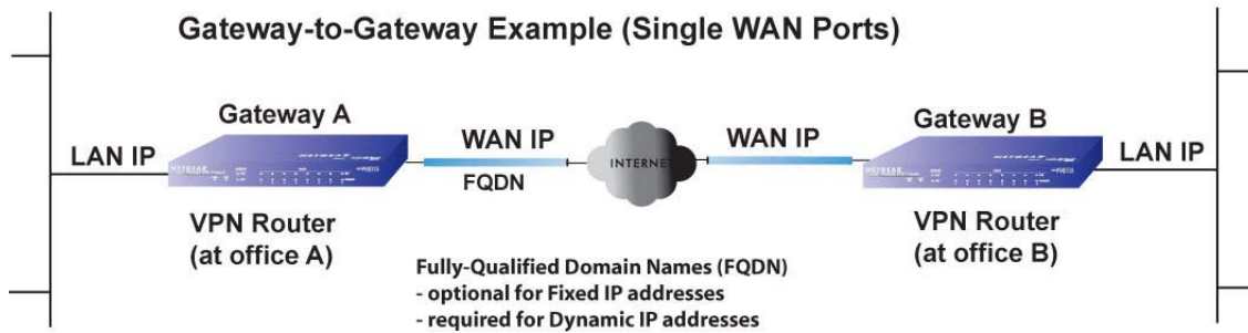
Figure 7. Example of an IPv4 gateway-to-gateway IPsec VPN connection
