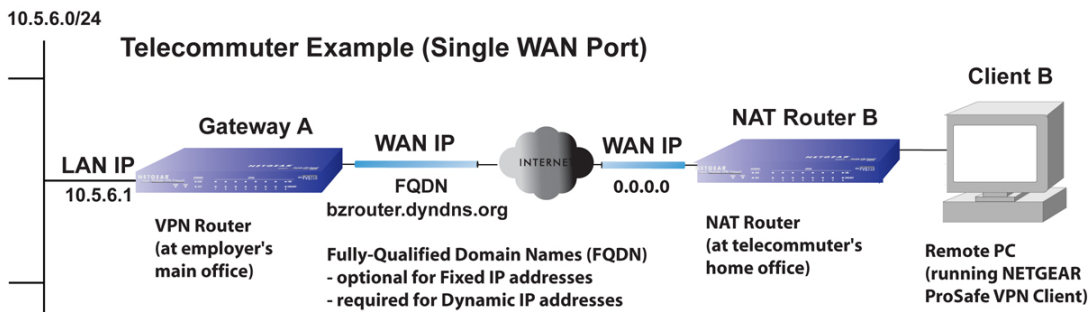
Figure 28. Telecommuter example in a single WAN port configuration with NAT
