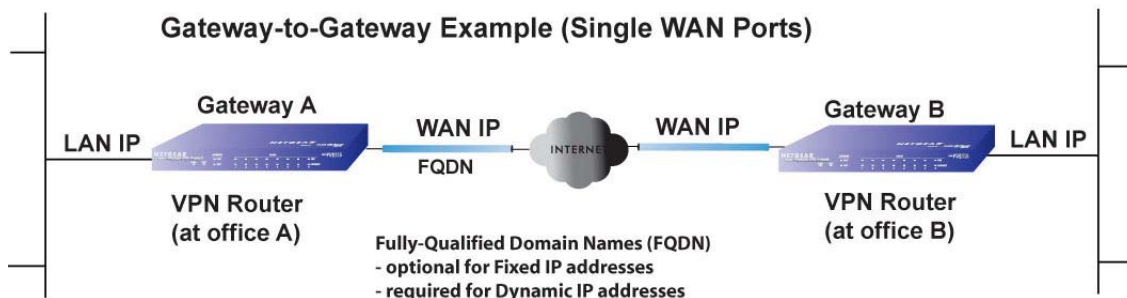
Figure 8. Example of an IPv6 gateway-to-gateway IPsec VPN connection
