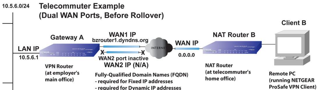
Figure 29. Telecommuter example in a dual WAN port configuration with NAT before auto-rollover
