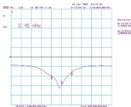
Return Loss
